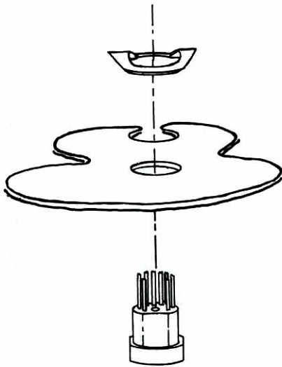
8-PIN SUB-MINIATURE SOCKET
