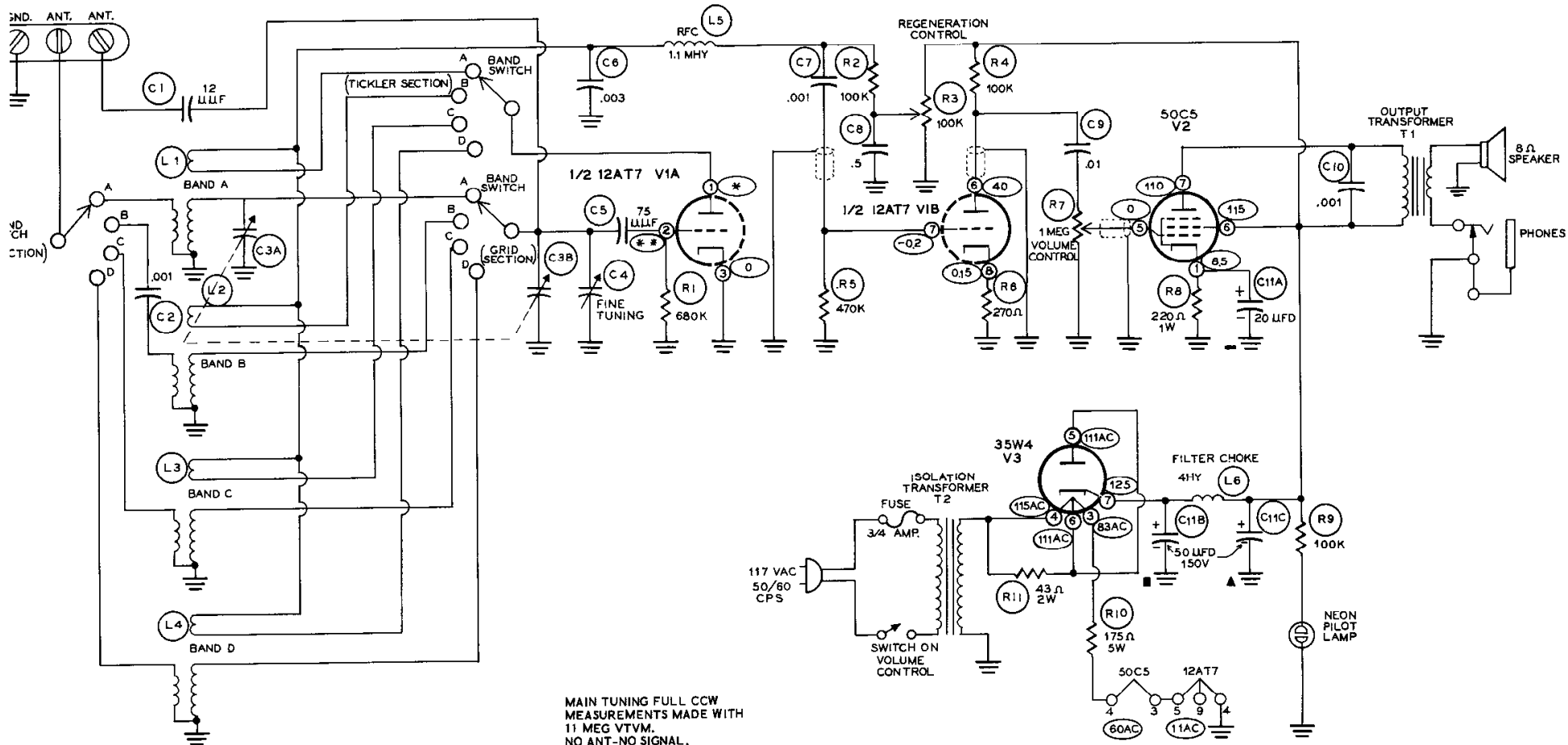
SCHEMATIC OF THE HEATHKIT® SHORT WAVE LISTENERS RADIO MODEL GR-81
